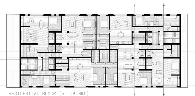
RESIDENTIAL BLOCK [RL +6.600]
