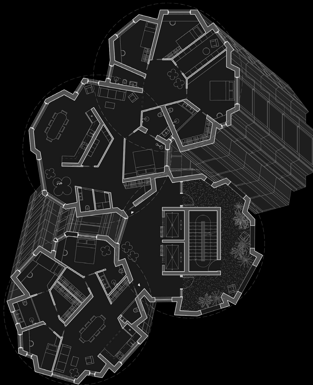
PL.3\ FLOOR PLAN
