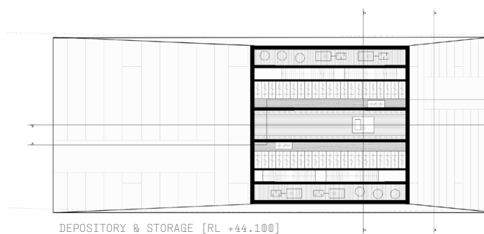
DEPOSITORY & STORAGE [RL +44.100]
