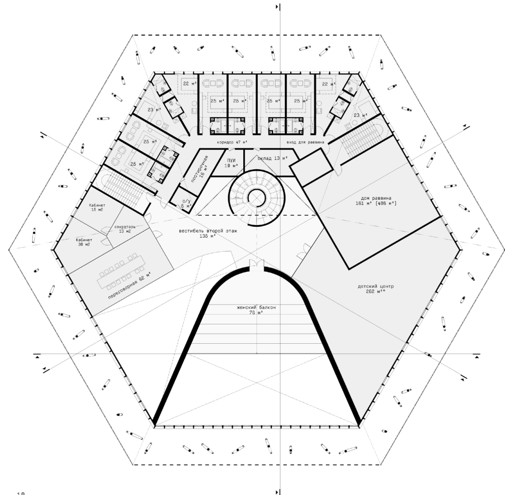
PL.5-6/ FLOOR PLANS
