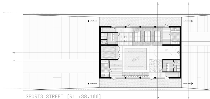
SPORTS STREET [RL +38.100]
